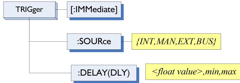
Figure 10- 10 TRIGger Subsystem Command Tree
