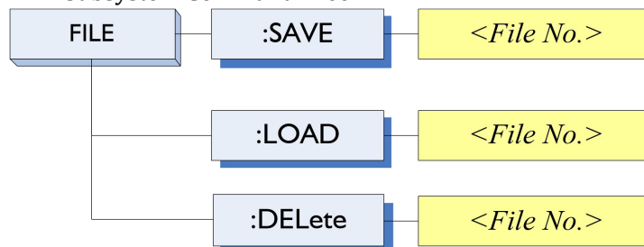
Figure 10-12 FILE Subsystem Command Tree
